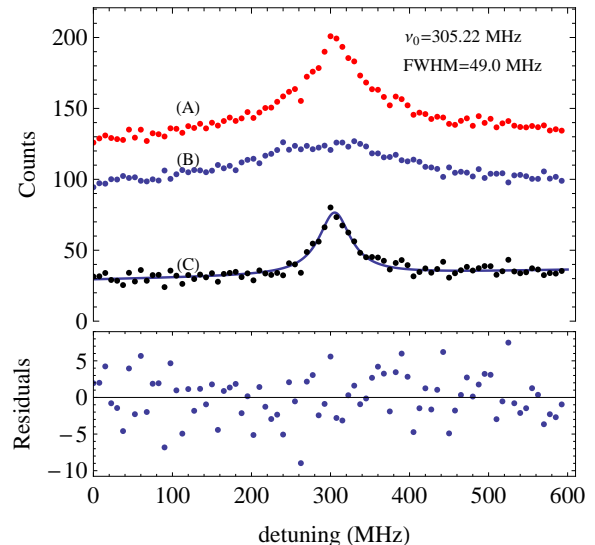
Figure 2: Typical fluorescence spectra obtained in an OODR run containing 44 laser scans. The scan direction is towards higher detuning. Upper graph: (A) Dark-count-rate reduced spectrum taken with all lasers on. (B) Spectrum obtained by summing the dark-count-rate reduced spectra taken with the parallel and antiparallel laser applied separately. Subtraction of spectrum (B) from (A) yields spectrum (C). The solid line reflects the fit of (C) by a Lorentzian together with a linear background. Lower graph: Residuals of the fit.
